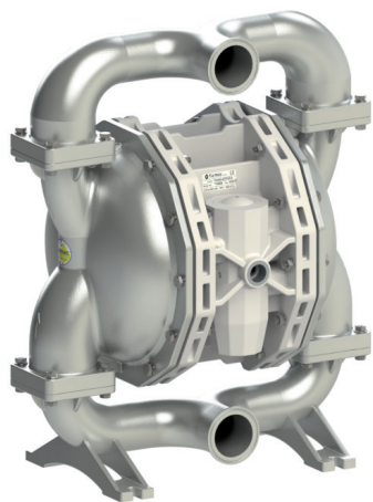
AISI 316 ELECTRO-POLISHED
